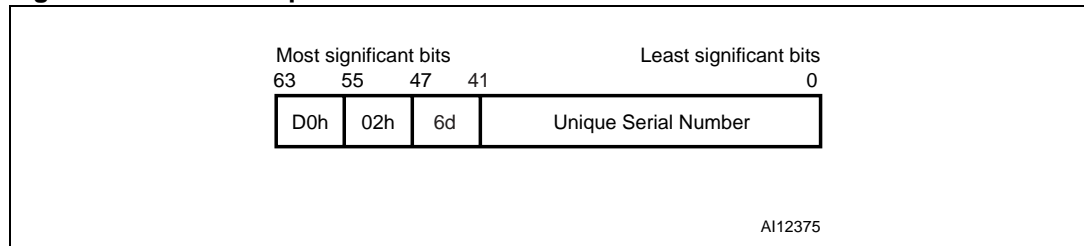
Figure 47. 64-bit unique identifier of SRT512
