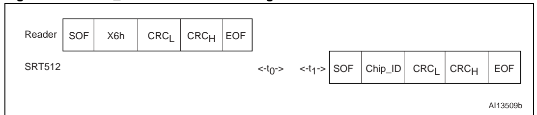
Figure 52. SLOT_MARKER frame exchange between Reader and SRT512
