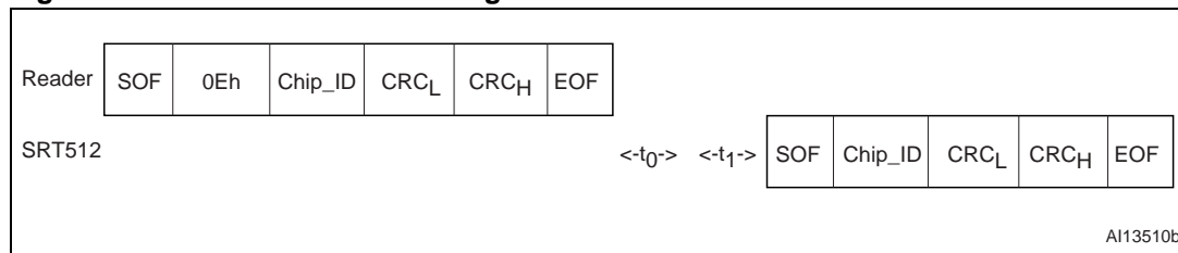
Figure 32. SELECT frame exchange between Reader and SRT512
