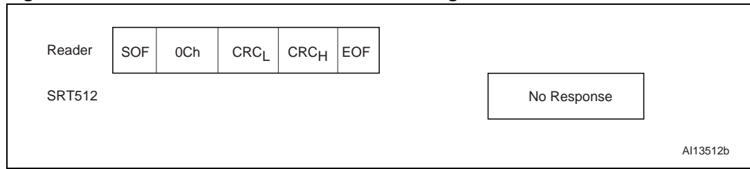
Figure 56. READ_BLOCK frame exchange between Reader and SRT512
