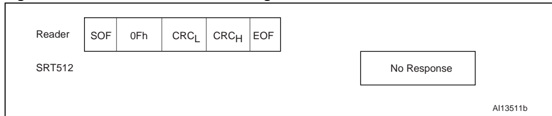
Figure 35. COMPLETION frame exchange between Reader and SRT512
