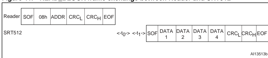
Figure 41. READ_BLOCK frame exchange between Reader and SRT512
