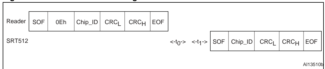
Figure 53. SELECT frame exchange between Reader and SRT512
