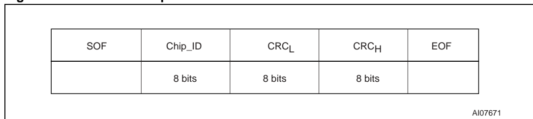
Figure 25. PCALL16 response format
