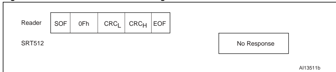
Figure 54. COMPLETION frame exchange between Reader and SRT512
