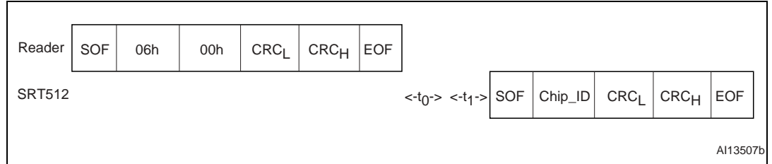
Figure 51. PCALL16 frame exchange between Reader and SRT512
