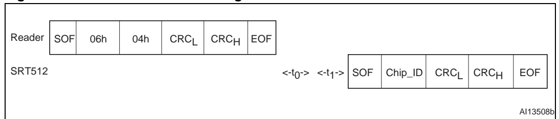
Figure 52. SLOT_MARKER frame exchange between Reader and SRT512
