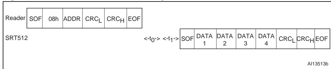
Figure 57. WRITE_BLOCK frame exchange between Reader and SRT512
