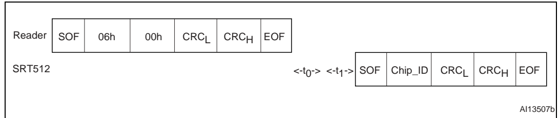
Figure 50. INITIATE frame exchange between Reader and SRT512
