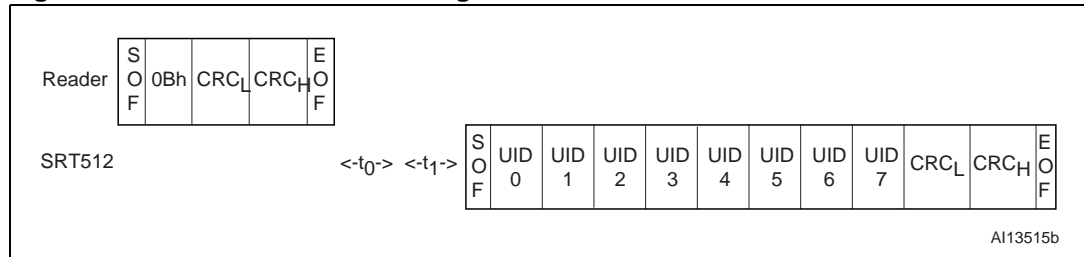
Figure 58. GET_UID frame exchange between Reader and SRT512
