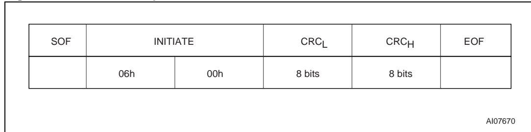
Figure 21. INITIATE request format
