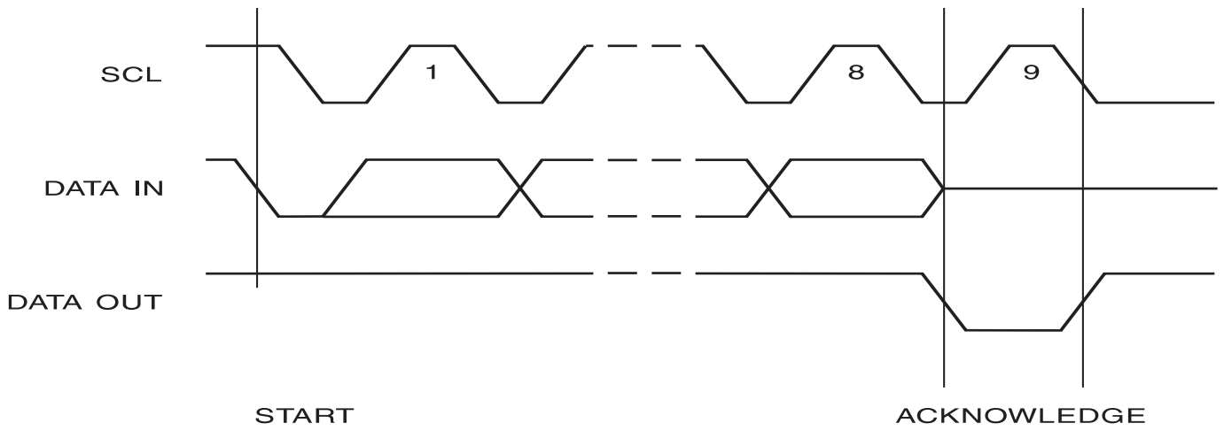
Figure 6. Output Acknowledge
